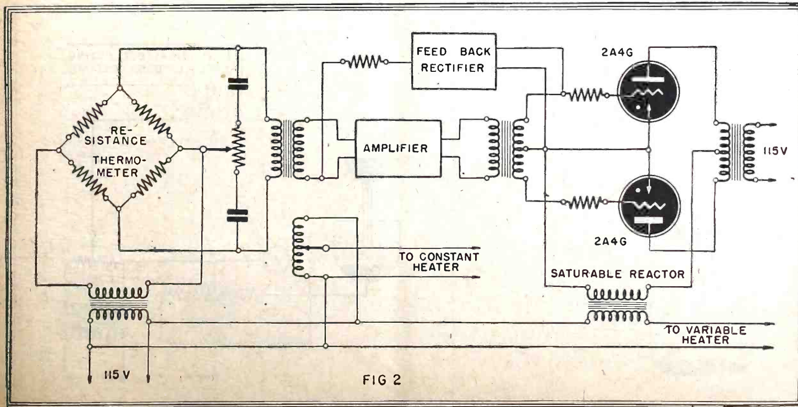
Fig. 2—An electronic control unit for furnaces. It uses a Wheatstone bridge, the resistance of two of the arms being varied by heat.
