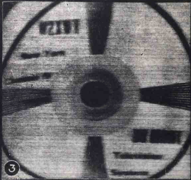
Figs. 1 and 2—The fixed ghost, and how it is formed. Fig. 3—A typical smear ghost. Figs. 4 and 5—How negative ghosts look.
